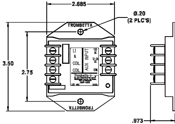
FIGURE #1 120 VAC AUX CONTROL
