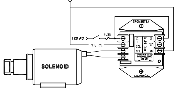
FIGURE #3 120 VAC LINE CONTROL
